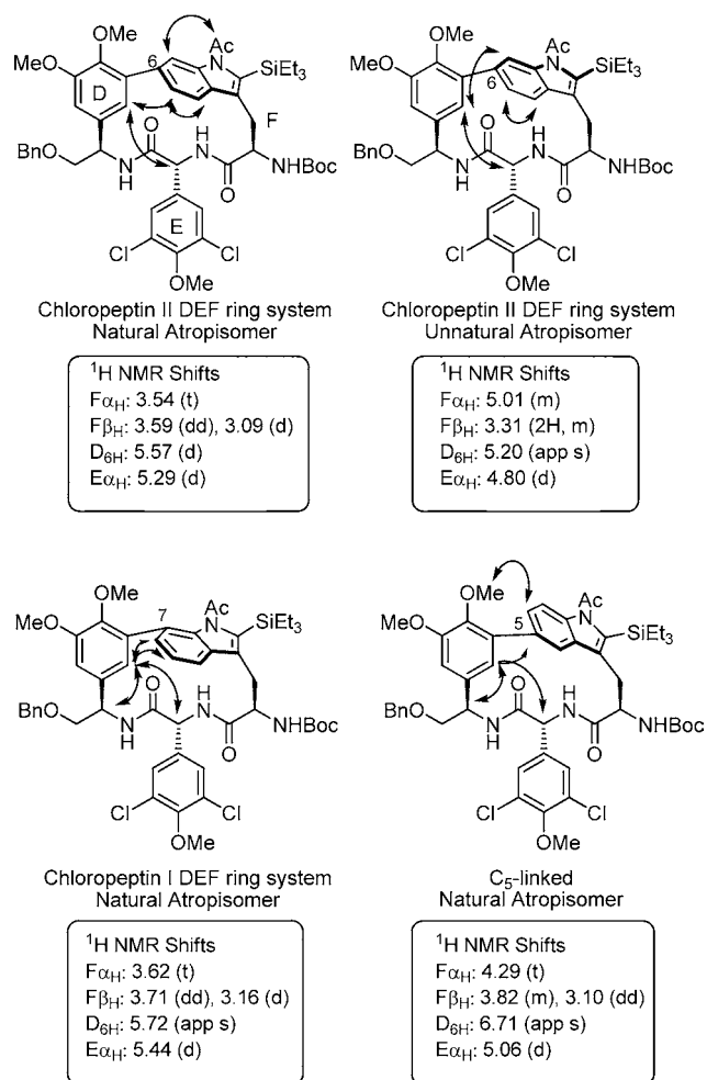
Figure 4. Diagnostic 1 H NMR chemical shifts and NOEs for indole macrocycles (CDCl 3 ).
